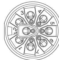
Cable connection side M12 (screw connection)
