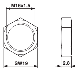
Dimensional drawing
