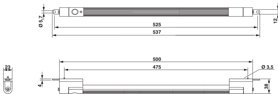
Dimensional drawing
