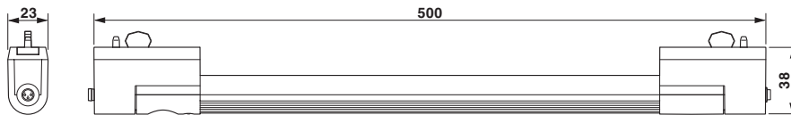
Dimensional drawing
