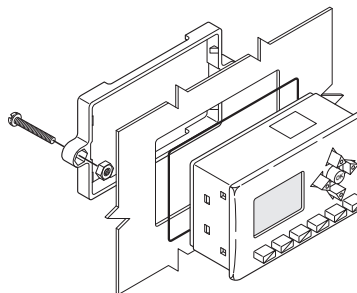
Schematic diagram
