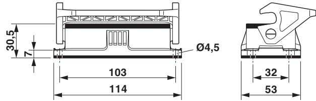
Dimensional drawing
